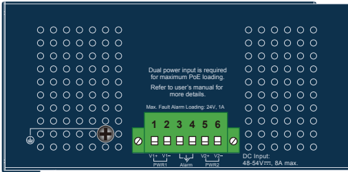
Figure 2-4: IGS-1000-8UP4X Upper Panel
