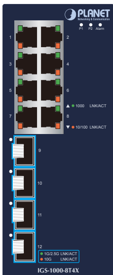
Figure 2-1: IGS-1000-8T4X front panel
