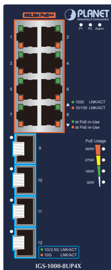
Figure 2-2: IGS-1000-8UP4X front panel
