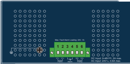
Figure 2-3: IGS-1000-8T4X Upper Panel.
